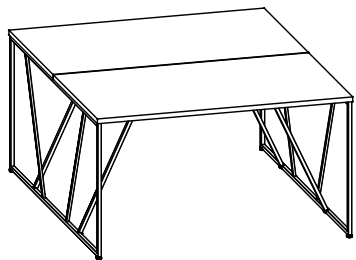
LWST 1316 1360x1606x750
